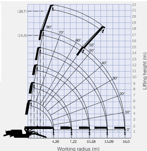
The Working Range Chart does not take into account boom deflection under load.
